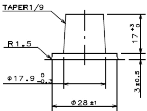
NEG TERMINAL
